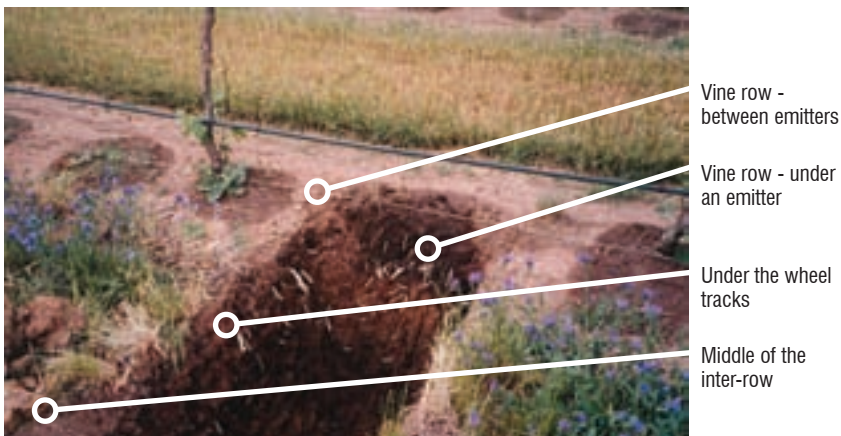
Figure 3.8. Soil sampling positions that take into account the patterns of variation in soil condition induced by a drip irrigation system (Source: McKenzie).
