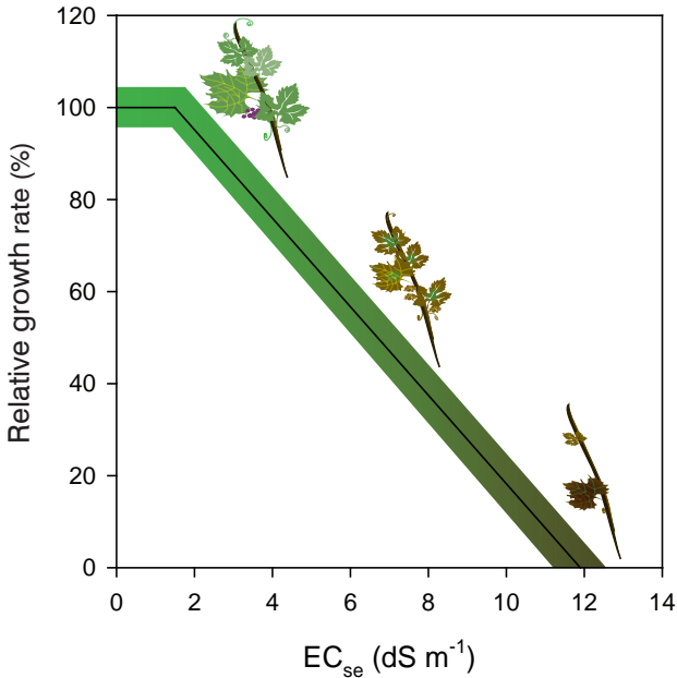
Figure 2.4. The relative response of vine growth to soil salinity ( EC_{se} ) where EC_{se} is the electrical conductivity of the saturated extract (Source: Mass and Hoffman 1977)
