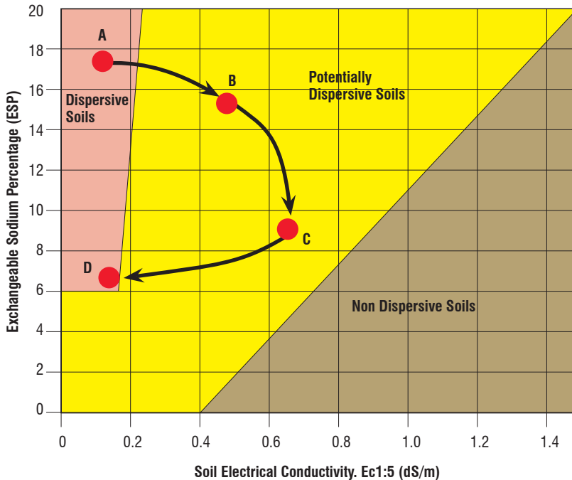
Figure 5.4. Prediction of the changes in dispersion and salinity characteristics with time after the initial application of 5 t/ha gypsum to the soil (adapted from Rengasamy et al. 1984). A. Initial condition of the soil, B. Increasing soil EC as gypsum dissolves into the soil water solution, C. Gypsum solubility reaches maximum and displaces the sodium ions with calcium ions leaving the sodium ions in solution, D. Winter rains leach the sodium ions from the soil profile thereby reducing salinity.
