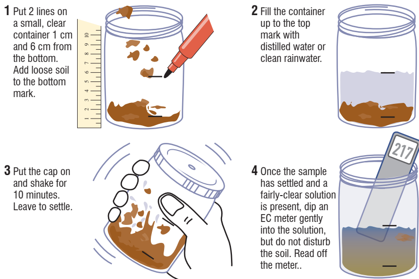
Figure 3.9. Rapid assessment of salinity in the field using a portable EC meter.
