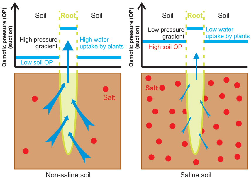
Figure 2.3. The relative water uptake by plants in saline and non-saline soils. In the saline soil the osmotic pressure associated with the salt reduces the pressure gradient between the soil and the root, reducing the flow of water into the root. This reduces the water available to the plant for growth and yield.
